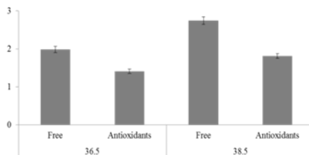
Fig. 3. Glutathione peroxidase (GSH-Px) activity of blastocysts obtained in vitro matured bovine oocytes at 36.5 or 38.5 °C free temperatures and cultured with antioxidants or antioxidants free embryo culture media after fertilization. The error bars represent the standard error of means and bars with different letters are significantly different at P < 0.05 .
